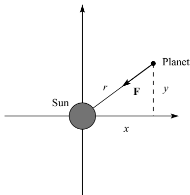
Figure 2.1.1. A planet under the gravitational attraction of the Sun.
